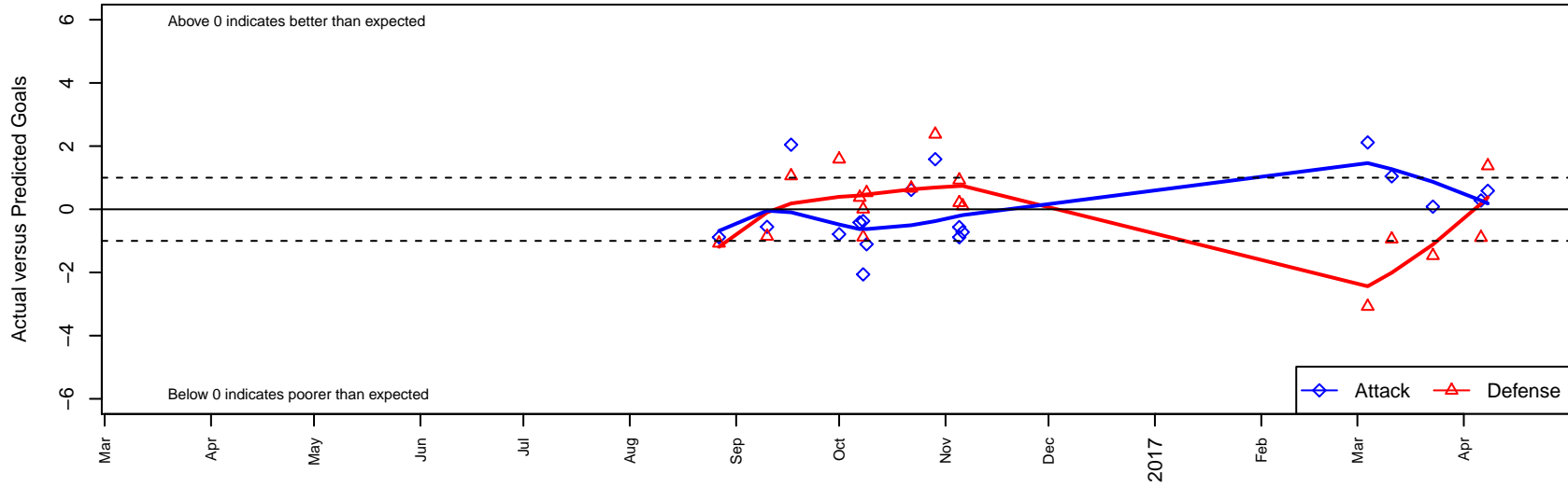
Idaho Arsenal United G04 Dots are actual minus expected GF (blue circles) and GA (red triangles). Blue line is smoothed change in attack strength. Red is smoothed change in defense strength.
